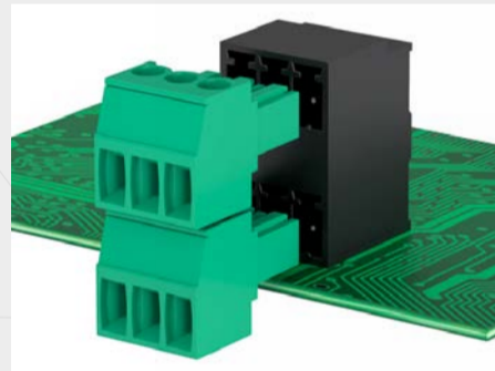
Wire insertion parallel to the PCB using screw type CTF series
