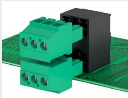
Wire insertion perpendicular to the PCB using screw type CKF series
