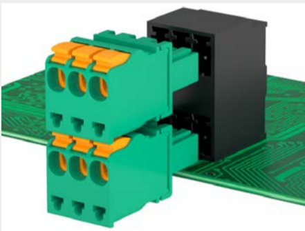
Push-in Technology using CBF plug series. Wire insertion parallel to the PCB
